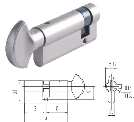
■ 标准K型卫生间锁芯 WASHROOM KNOB CYLINDER MODEL B
