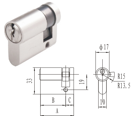
■ 半个锁芯 PROFILE HALF CYLINDER
