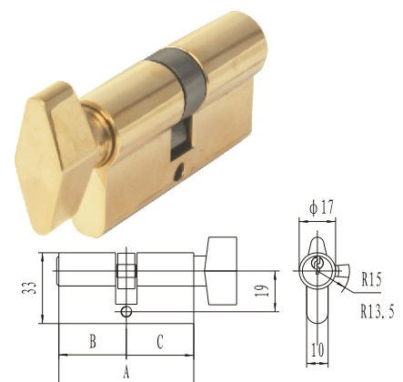
■ 标准A型手轮锁芯 PROFILE KNOB CYLINDER MODEL B
